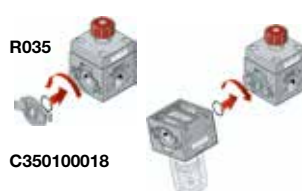
R035 assembly with connecting clips C350100018
